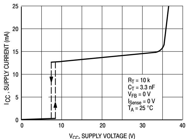
Figure 17. Supply Current versus Supply Voltage
