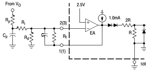
Figure 32. Error Amplifier Compensation
