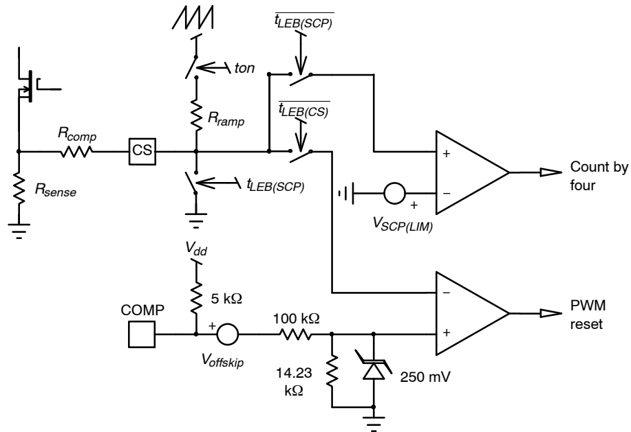
Figure 45. If the Current Sense Pin Exceeds the Maximum Cycle-by-cycle Limit by 25%, a Counter Records the Event and Stops All Pulses after 4 Consecutive Events
