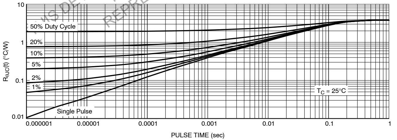
Figure 16. Thermal Response
