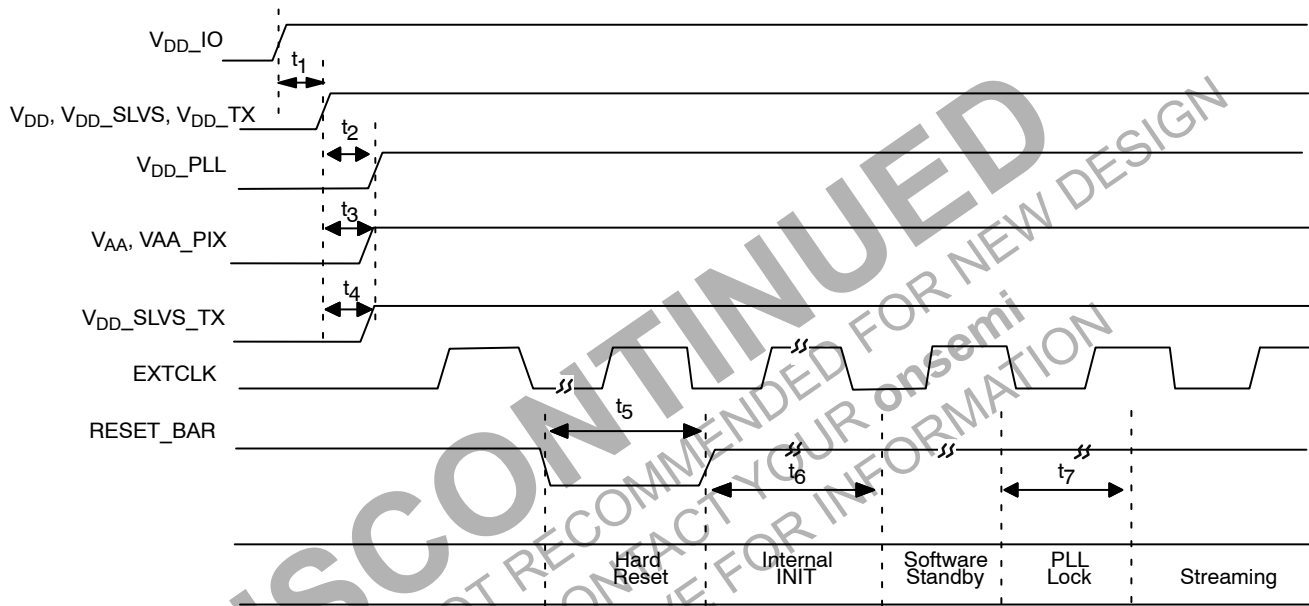
Figure 45. Power-Up Sequence
