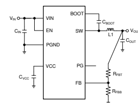
Simplified Schematic
