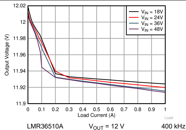
Figure 8-9. Load Regulation
