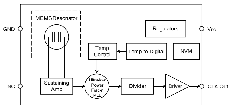
Figure 2. SiT1581 Block Diagram
