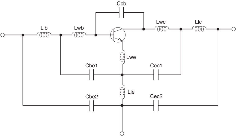
Figure 10. Schematic
