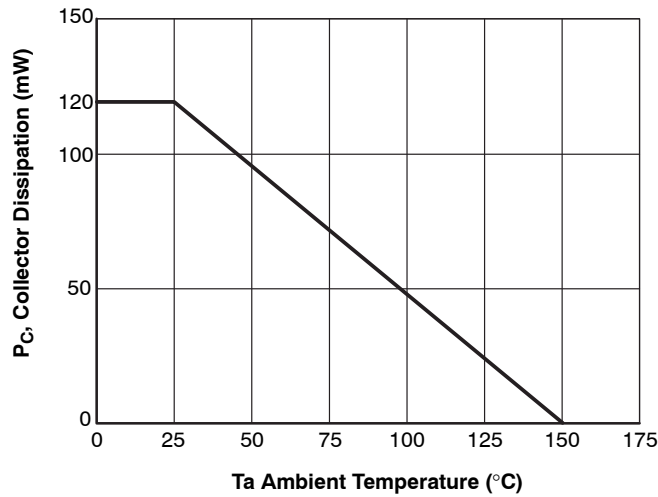
Figure 9. P_C – T_a
