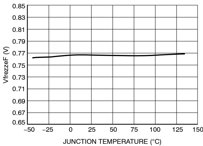
Figure 21. VfreeF vs. Junction Temperature
