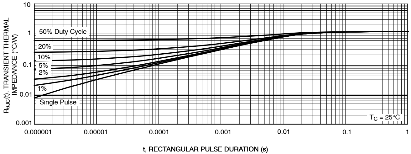
Figure 14. Thermal Response
