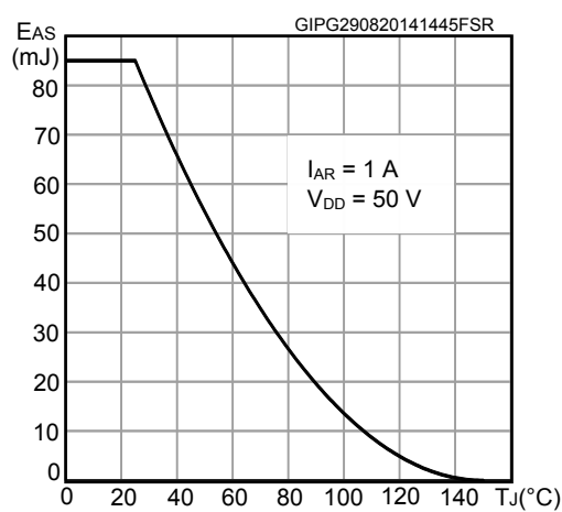
Figure 11. Maximum avalanche energy vs starting TJ
