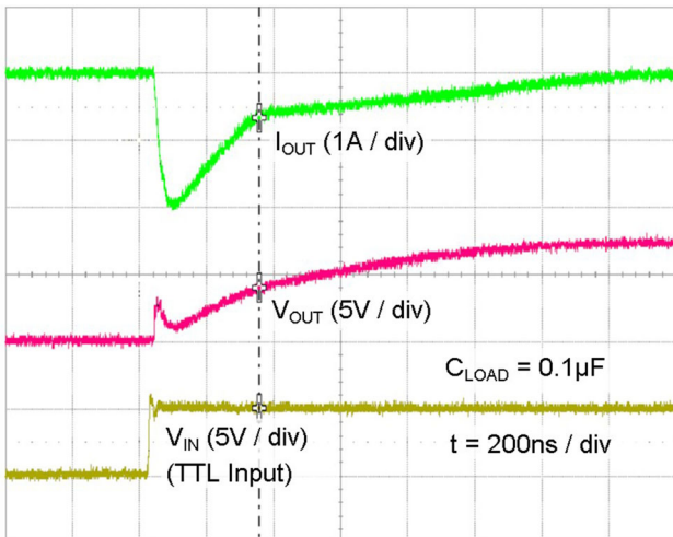
Figure 35. Quasi-Static Source Current with V_{DD} = 8 V
