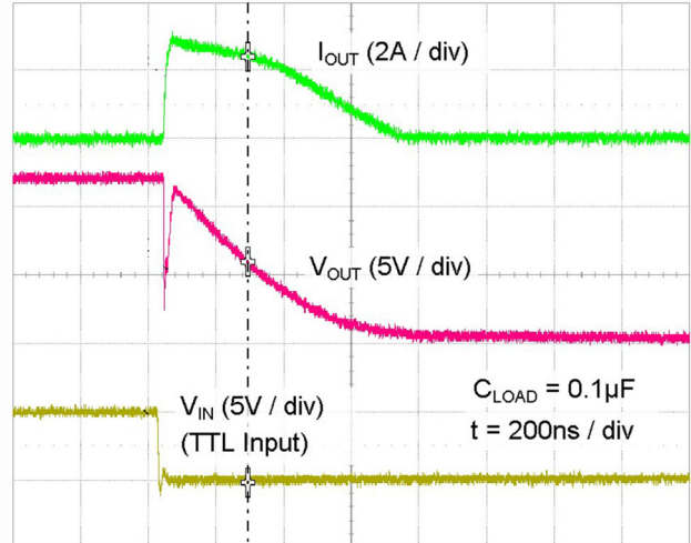
Figure 34. Quasi-Static Sink Current with V_{DD} = 12 V
