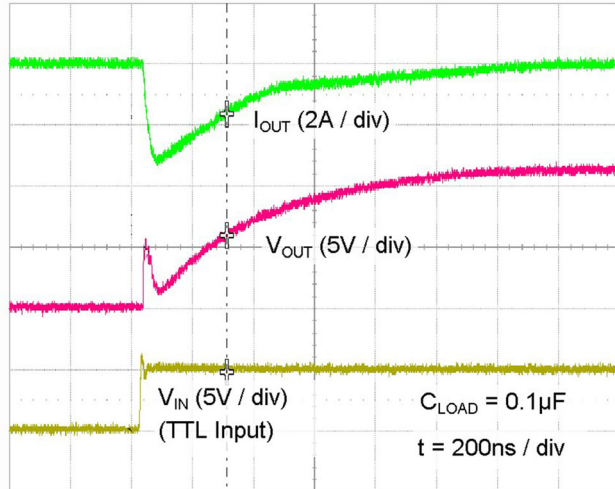
Figure 33. Quasi-Static Source Current with V_{DD} = 12 V
