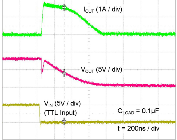
Figure 36. Quasi-Static Sink Current with V_{DD} = 8 V
