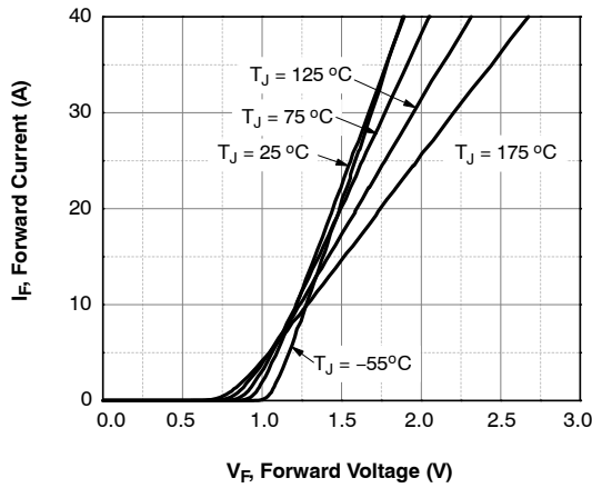
Figure 1. Forward Characteristics
