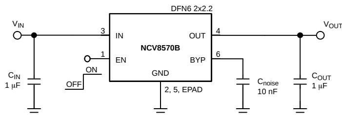
Figure 1. NCV8570B Typical Application Schematic
