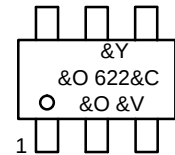
TSOT23 6-Lead CASE 419BL
