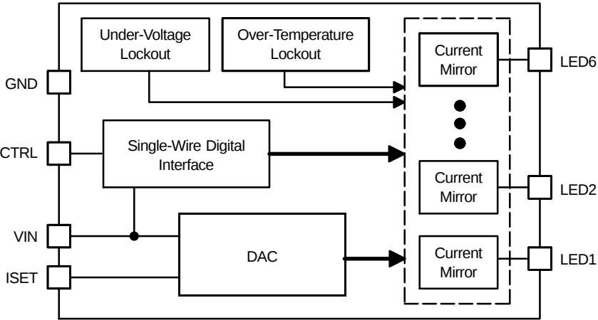
Figure 4. Block Diagram
