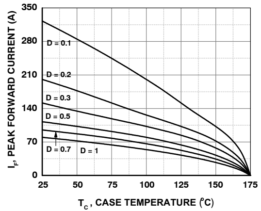
Figure 4. Current Derating
