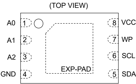
Figure 3-(b). Pin Configuration (VSON008X2030*1, VSON08AX2030)
