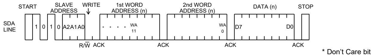
Figure 41. Byte Write
