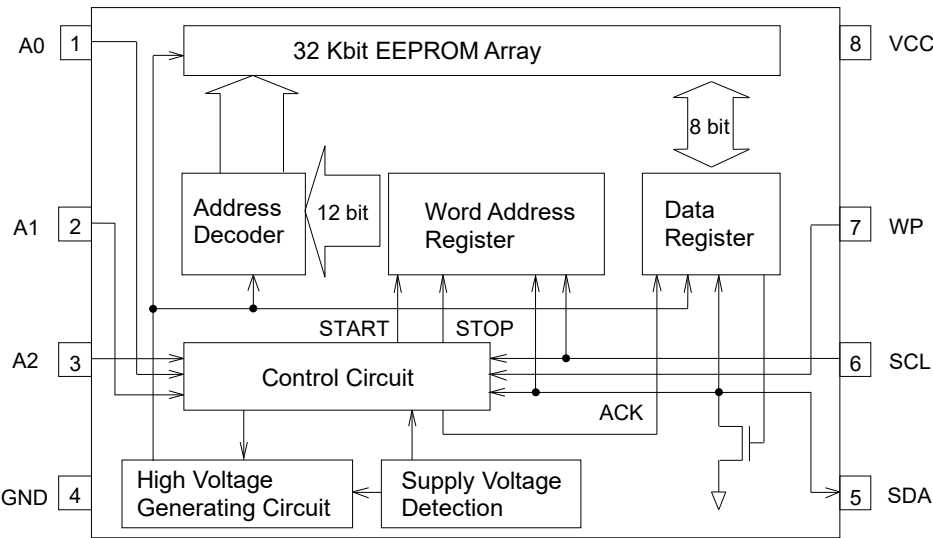
Figure 4. Block Diagram
