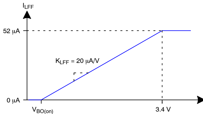
Figure 45. Transfer Function of the Line Feed Forward
