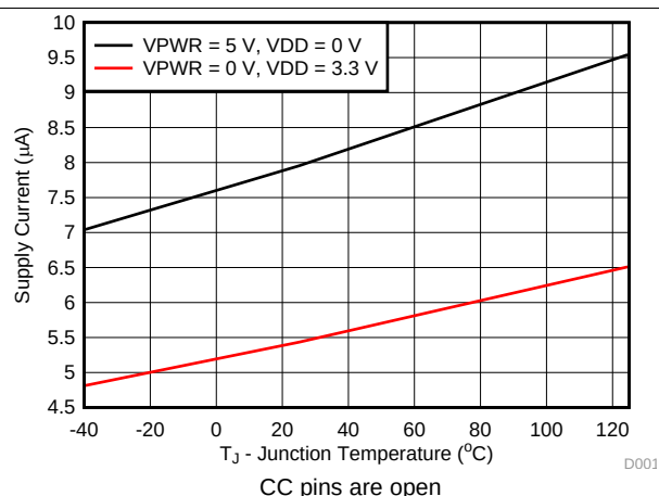
Figure 9. Supply Current when V_{PWR} = 5 V
