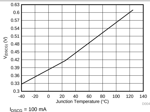
Figure 7. V_{DSCG} when V_{PWR} > 4.65 V
