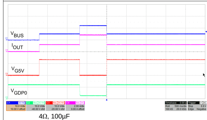
Figure 56. VBUS 5 V – 12 V – 5 V Transition, TPS25741
