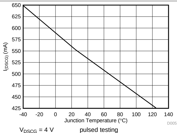
Figure 8. I_{DSCG} when V_{PWR} > 4.65 V
