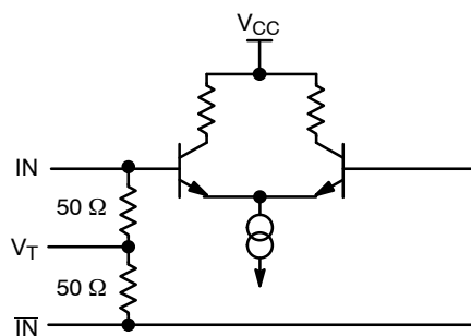
Figure 3. Input Structure
