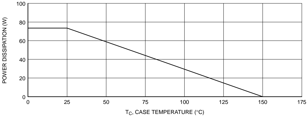
Figure 14. Power vs. Case Temperature
