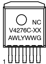
D 2 PAK 5-PIN DS SUFFIX CASE 936A
