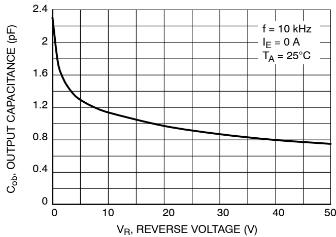
Figure 14. Output Capacitance
