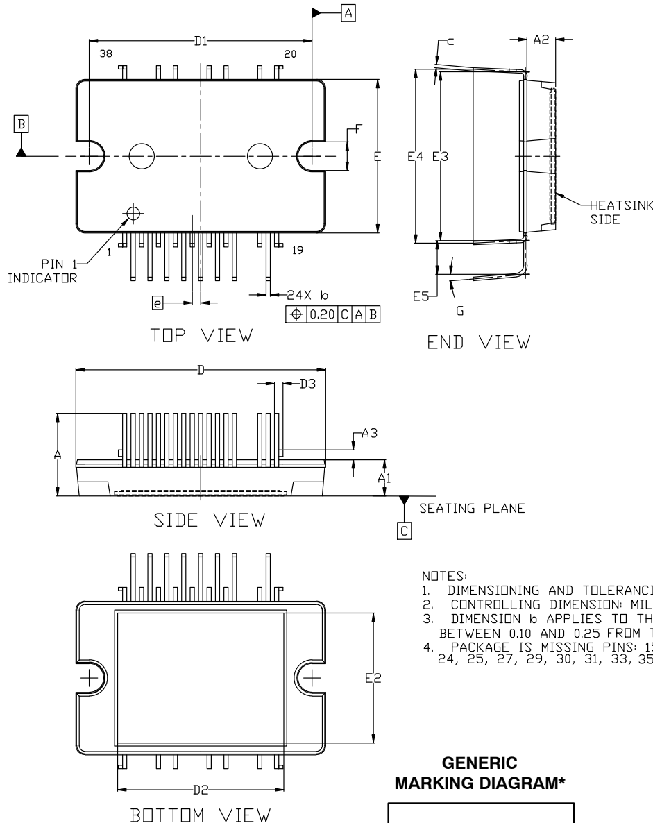
DIP38, 29.60x18.20x9.80, 1.00P (EP-5) CASE 181AE ISSUE B
