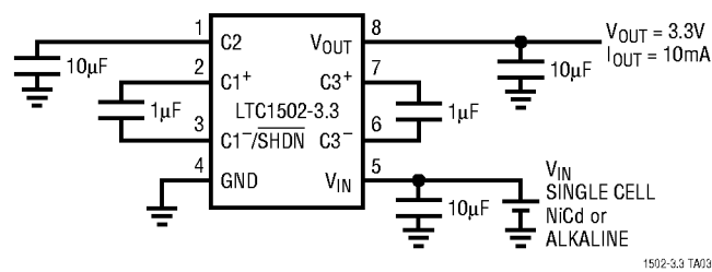
Minimum Component Count Single Cell 3.3V Regulated Supply
