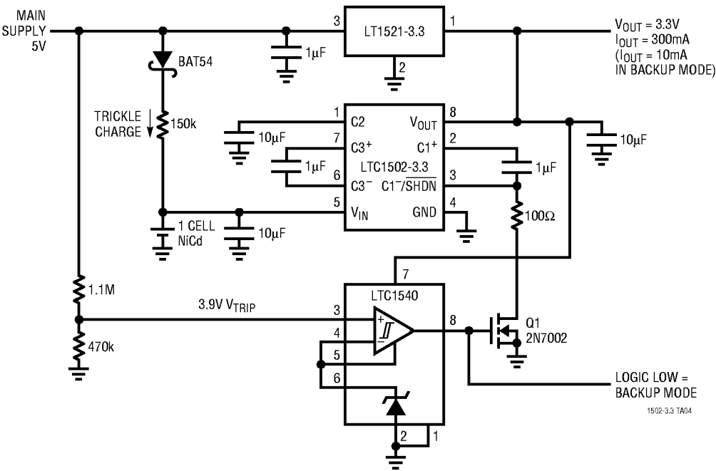
Single Cell Battery Backup Supply with Autoswitchover and No Reverse Current
