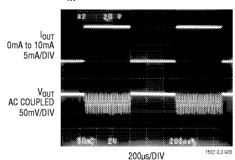
Load Transient Response V_{IN} = 1.25\text{V}
