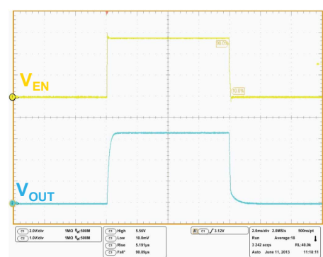
Figure 29. Turn-on time
