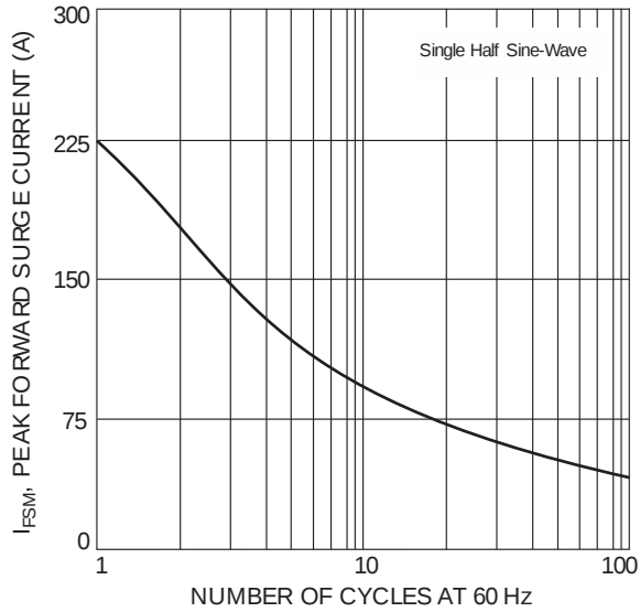
Figure 3 Forward Surge Current Derating Curve
