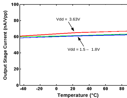
Output Stage Current over Temperature
