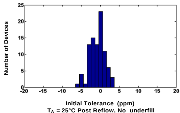
Initial Tolerance Histogram
