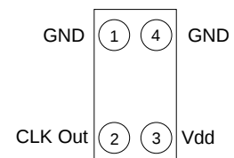
CSP Package (Top View)
