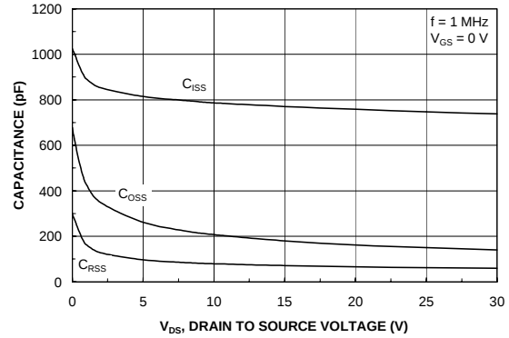
Figure 18. Capacitance Characteristics.
