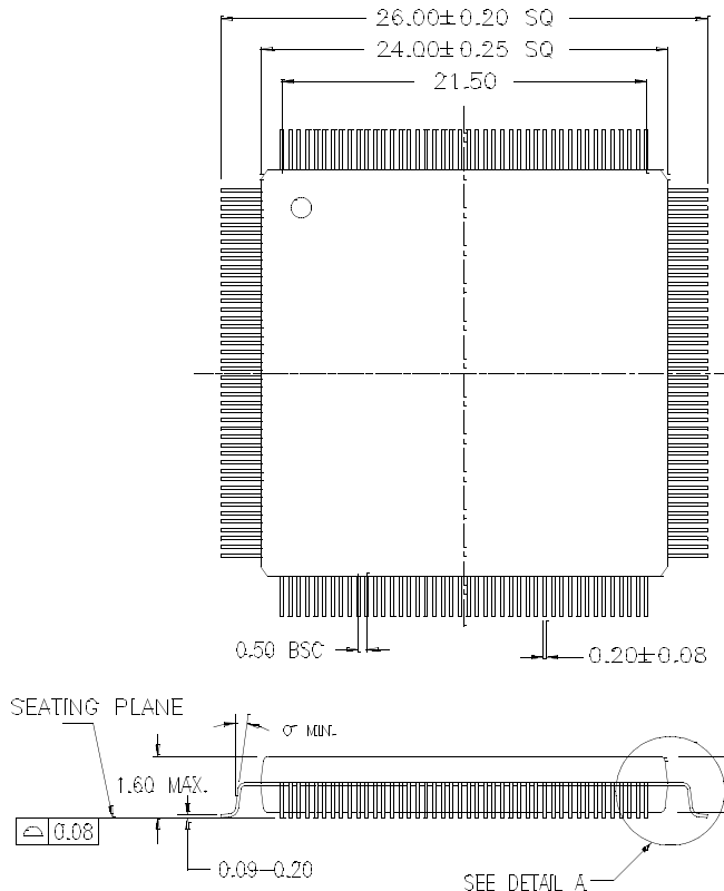
176-lead Thin Quad Flat Pack (24 × 24 × 1.4 mm) A176
