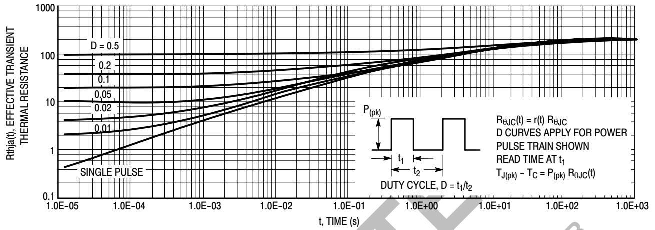
Figure 16. Thermal Response
