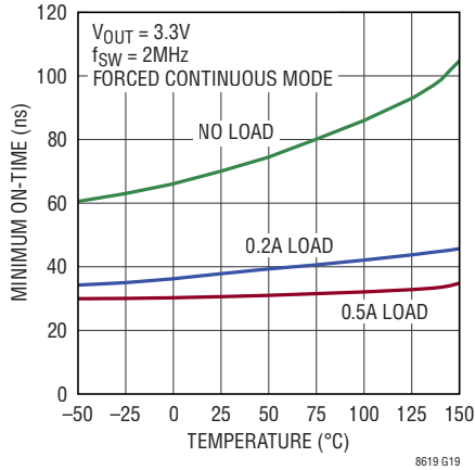
Minimum On-Time
