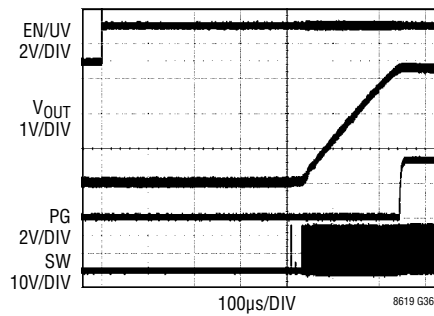
EN/UV Start-Up
