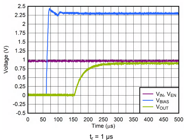
Figure 6-17. Start-Up With V_{\text{IN}} and V_{\text{EN}} Before V_{\text{BIAS}}
