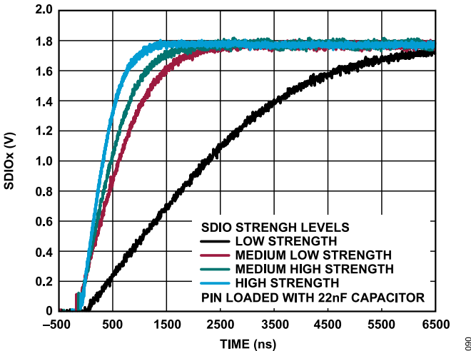
Figure 86. Driving Strength Options
