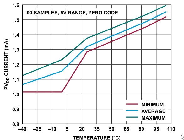
Figure 67. PV_{DD} Current vs. Temperature
