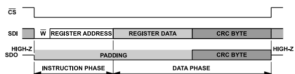
Figure 79. Basic SPI Write Frame with CRC
