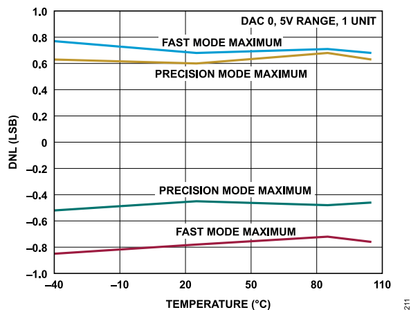
Figure 20. DNL vs. Temperature
