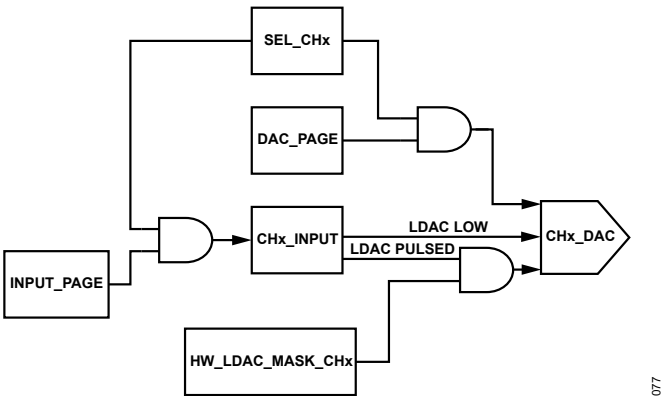
Figure 87. DAC Data Flow Between Registers
