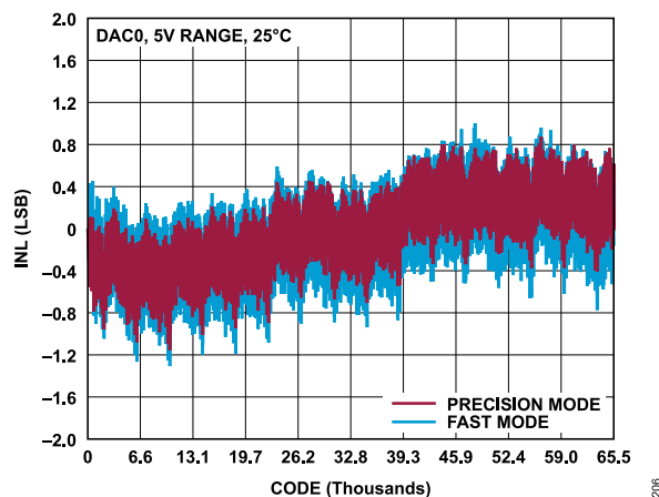
Figure 15. INL vs. Code, 0 V to 5 V Range, 25^\circ\text{C} , Fast Mode and Precision Mode
