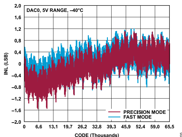
Figure 14. INL vs. Code, 0 V to 5 V Range, -40^\circ\text{C} , Fast Mode and Precision Mode
