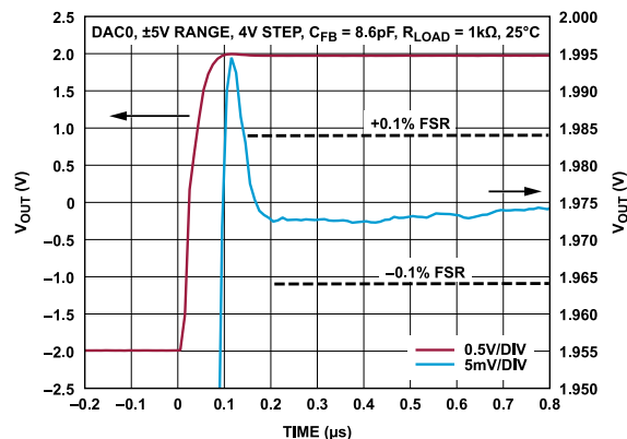
Figure 55. Large Signal Settling Time, -5 V to +5 V Range
