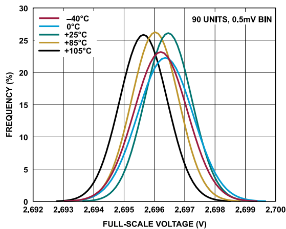
Figure 40. Full-Scale Voltage Distribution, 0 V to 2.5 V Range
