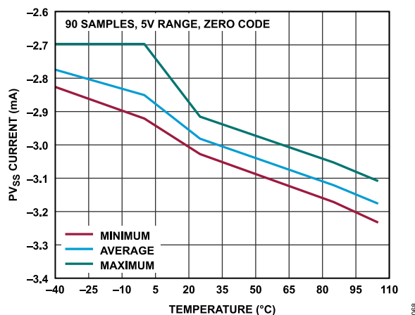
Figure 68. PV_{SS} Current vs. Temperature
