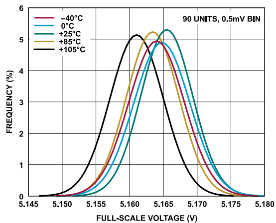
Figure 43. Full-Scale Voltage Distribution, -5 V to +5 V Range
