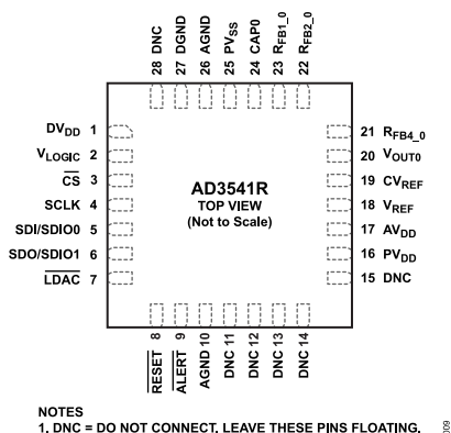
Figure 9. Pin Configuration
