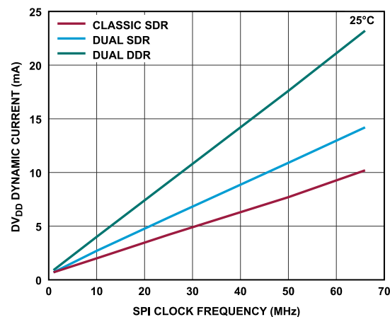
Figure 63. DV_{DD} Dynamic Current vs. SPI Clock Frequency, SPI Mode
