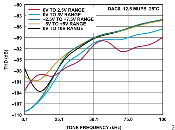
Figure 30. THD vs. Tone Frequency
