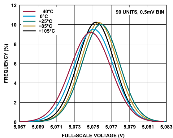
Figure 41. Full-Scale Voltage Distribution, 0 V to 5 V Range
