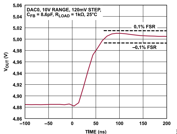
Figure 51. Small Signal Settling Time, 0 V to 10 V Range
