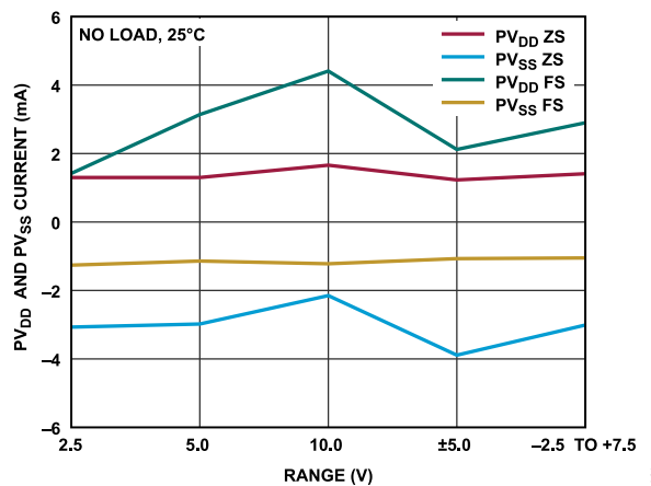
Figure 69. PV_{DD} and PV_{SS} Current vs. Range
