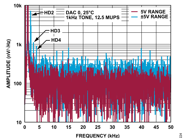
Figure 33. Spectral Noise Density with 1 kHz Sine Wave Playback (HD2 Is Second Harmonic Distortion, HD3 Is Third Harmonic Distortion, HD4 Is Fourth Harmonic Distortion)
