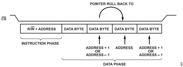
Figure 78. Looping Enabled with STREAM_MODE = 2
