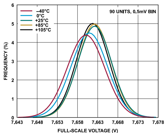
Figure 44. Full-Scale Voltage Distribution, -2.5 V to +7.5 V Range
