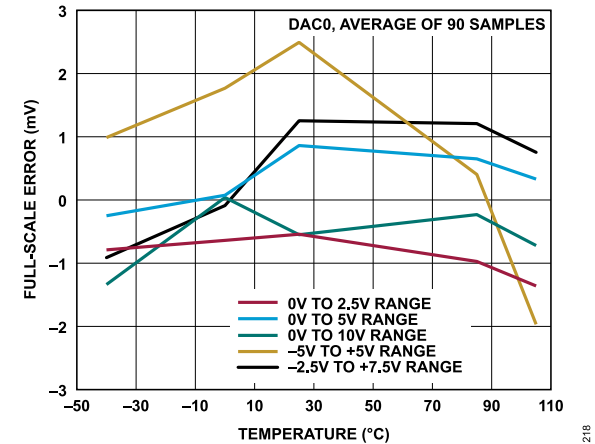
Figure 27. Full-Scale Error vs. Temperature
