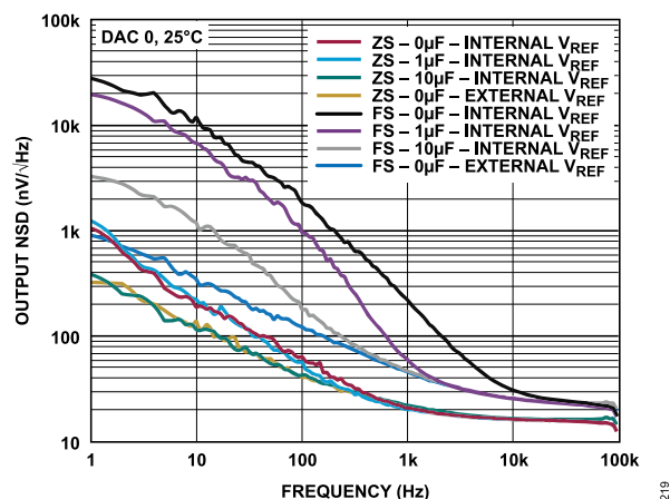
Figure 28. Output Noise Spectral Density (NSD) vs. Frequency
