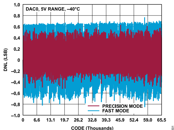
Figure 10. DNL vs. Code, 0 V to 5 V Range, -40^\circ\text{C} , Fast Mode and Precision Mode
