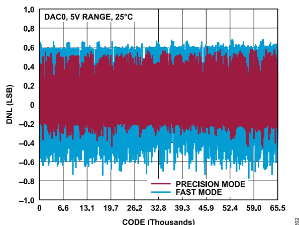
Figure 11. DNL vs. Code, 0 V to 5 V Range, 25^\circ\text{C} , Fast Mode and Precision Mode
