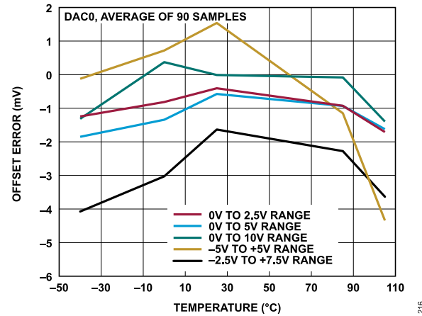
Figure 25. Offset Error vs. Temperature
