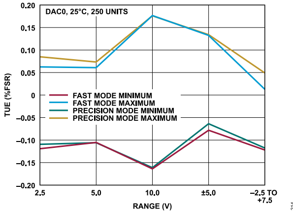
Figure 23. TUE vs. Range
