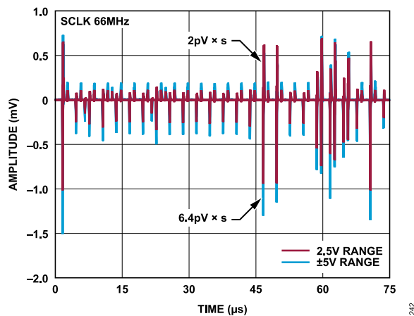
Figure 49. Digital Feedthrough
