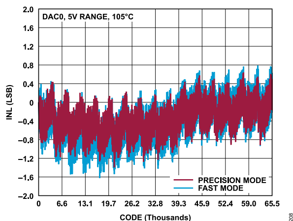
Figure 17. INL vs. Code, 0 V to 5 V Range, 105°C, Fast Mode and Precision Mode
