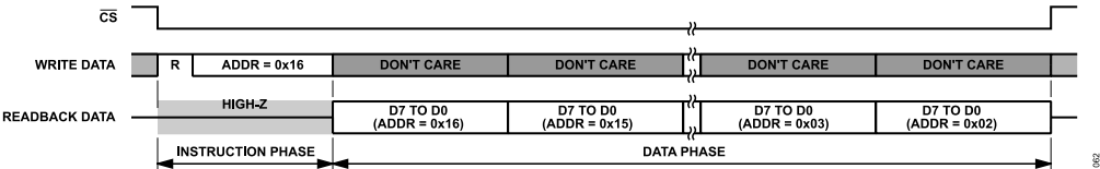
Figure 77. Streaming Mode Register Read with Looping Disabled
