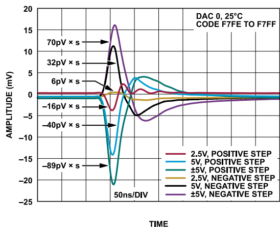
Figure 47. Digital-to-Analog Glitch
