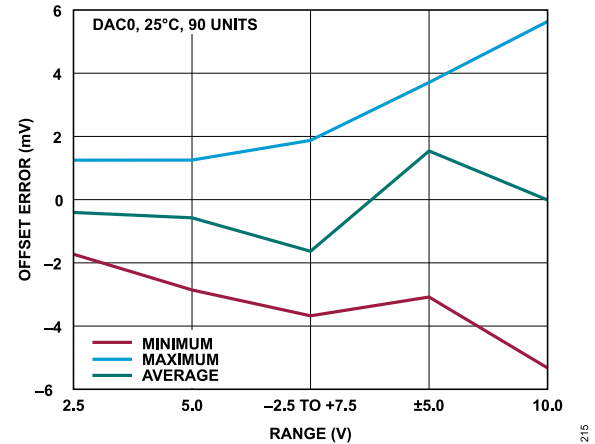
Figure 24. Offset Error vs. Range
