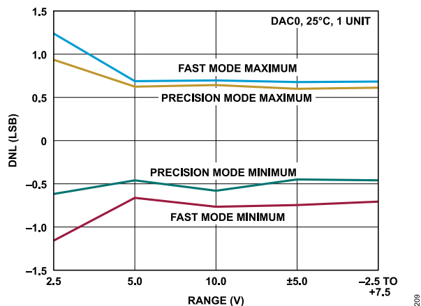
Figure 18. DNL vs. Range, Fast Mode and Precision Mode
