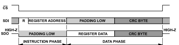
Figure 80. Basic SPI Read Frame with CRC
