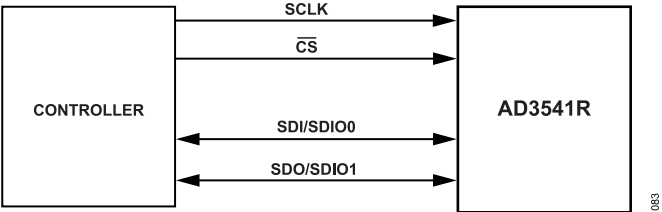
Figure 83. Dual SPI Connection
