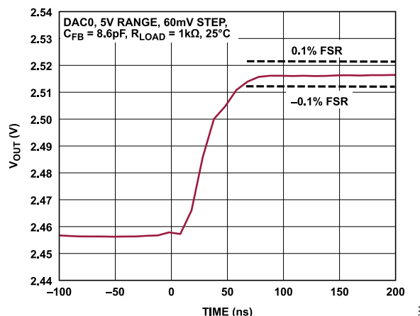
Figure 50. Small Signal Settling Time, 0 V to 5 V Range ( R_{LOAD} Is Load Resistance)
