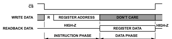
Figure 72. Basic SPI Read Frame
