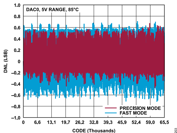
Figure 12. DNL vs. Code, 0 V to 5 V Range, 85^\circ\text{C} , Fast Mode and Precision Mode
