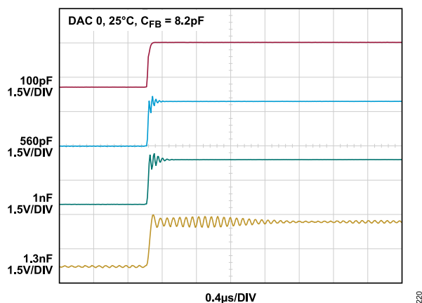
Figure 29. Output Load Stability ( C_{FB} Is Feedback Capacitor)
