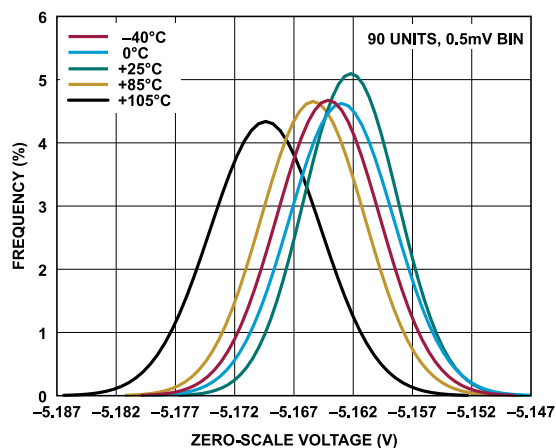
Figure 38. Zero-Scale Voltage Distribution, -5 V to +5 V Range
