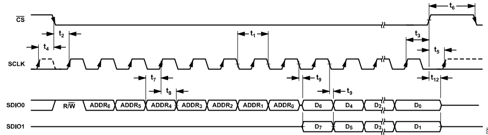
Figure 6. Dual SPI Read Operation with Single Data Rate
