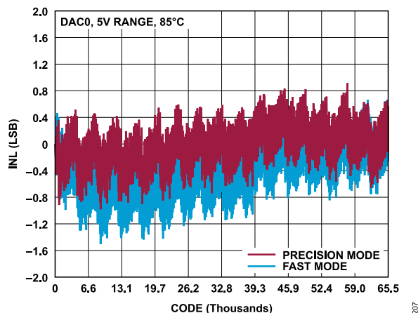
Figure 16. INL vs. Code, 0 V to 5 V Range, 85°C, Fast Mode and Precision Mode
