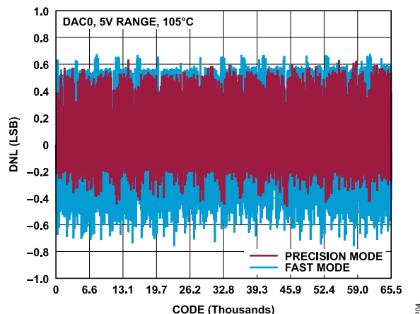
Figure 13. DNL vs. Code, 0 V to 5 V Range, 105^\circ\text{C} , Fast Mode and Precision Mode
