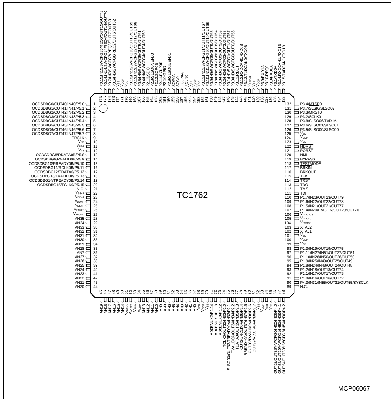
Figure 2-3 TC1762 Pinning for PG-LQFP-176-2 Package
