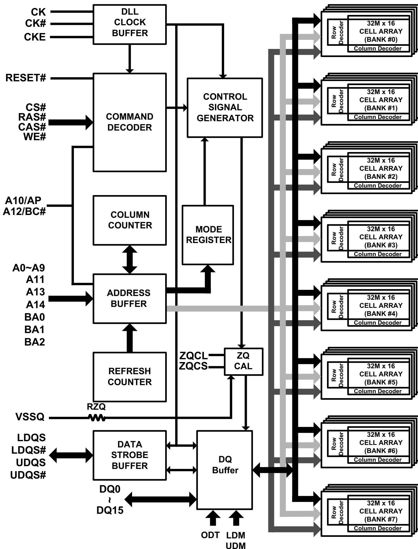
Figure 2. Block Diagram
