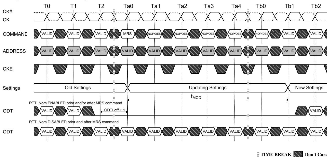
Figure 7. t_{MOD} timing
