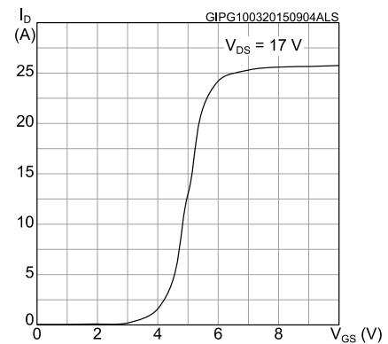
Figure 7: Transfer characteristics
