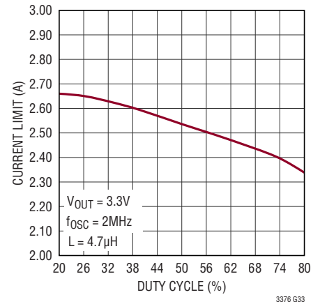
1.5 Buck Current Limit vs Duty Cycle
