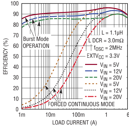
6A Buck Efficiency vs I_{\text{LOAD}} , V_{\text{OUT}} = 3.3\text{V}
