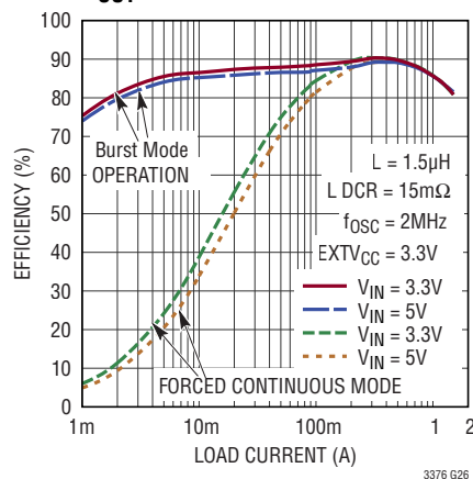
1.5A Buck Efficiency vs I_{\text{LOAD}} , V_{\text{OUT}}=1.2\text{V}
