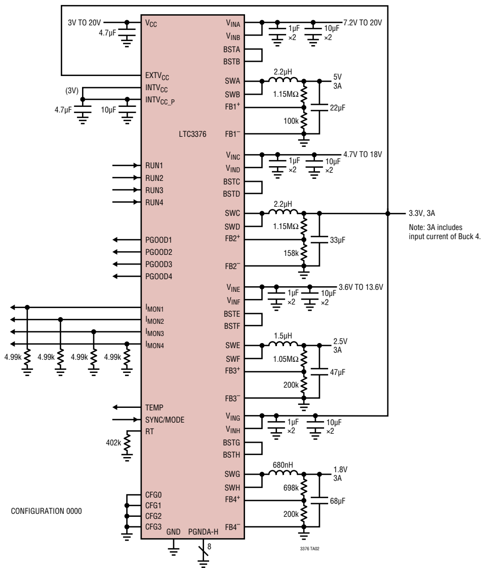
Four Rail (5V/3.3V/2.5V/1.8V, 3A) System with Bootstrapped EXTV CC Drive
