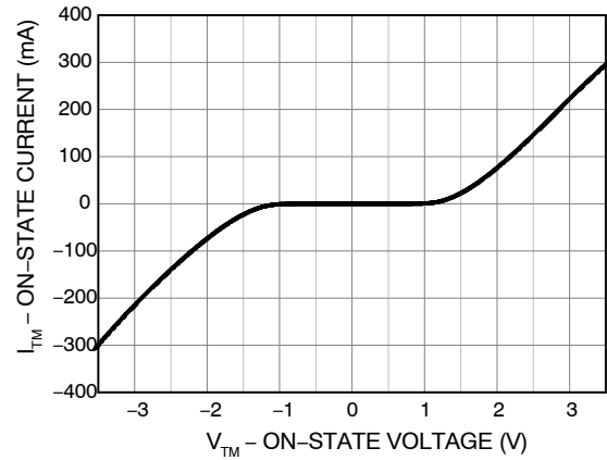
Figure 2. On-State Characteristics
