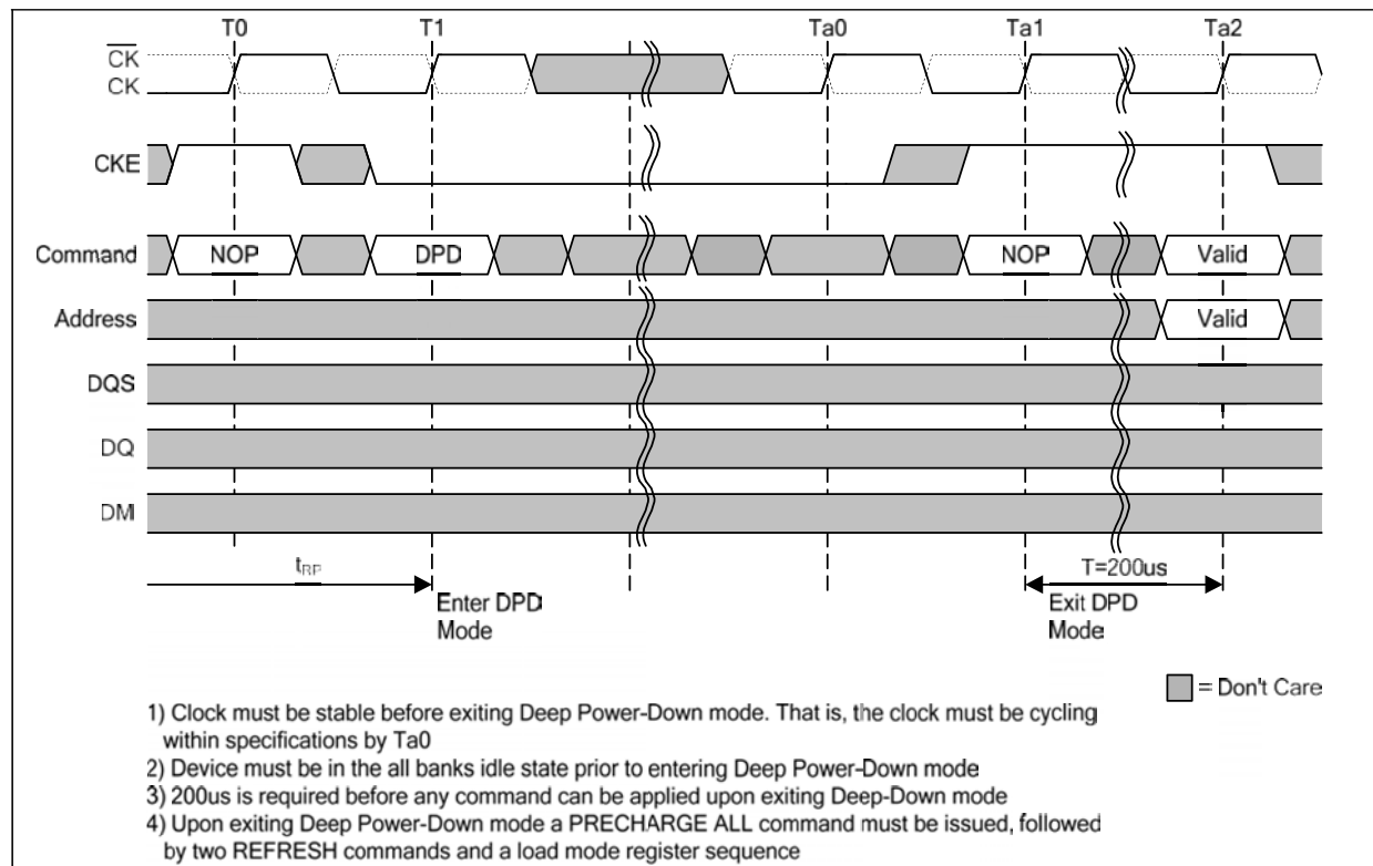
Figure 38 — Deep Power-Down Entry and Exit
