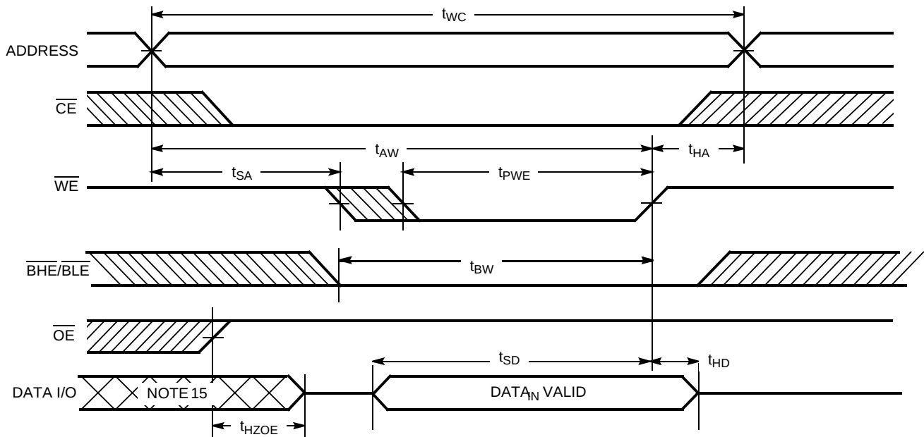
Write Cycle No. 1 ( \overline{\text{WE}} Controlled) [8, 13, 14]
