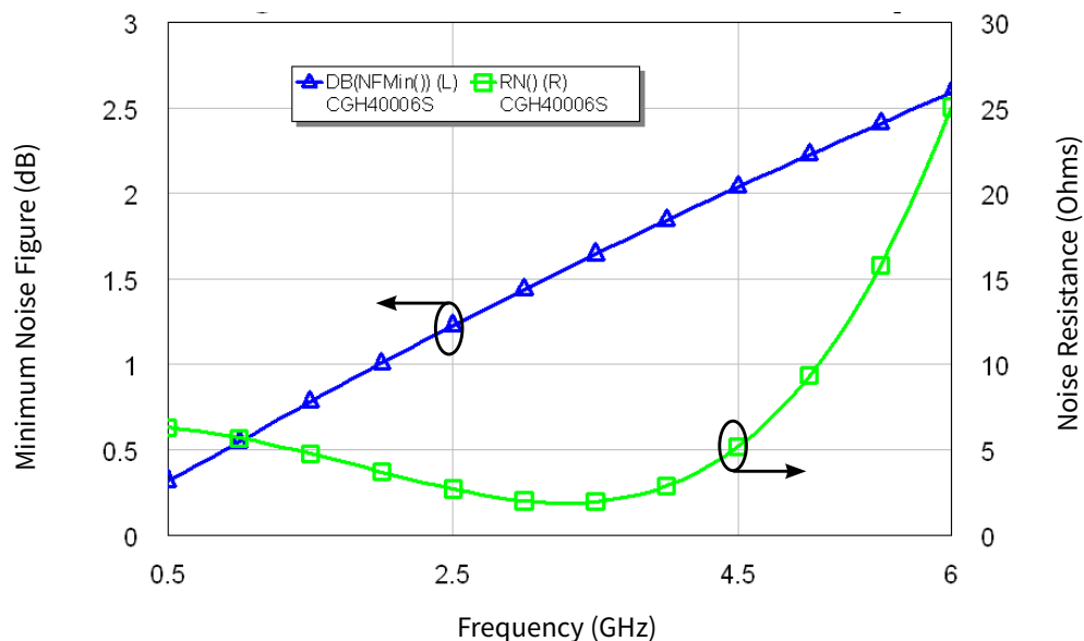
Figure 12. Simulated Minimum Noise Figure and Noise Resistance vs Frequency of the CGH40006S V_{DD} = 28\text{ V} , I_{DQ} = 100\text{ mA}
