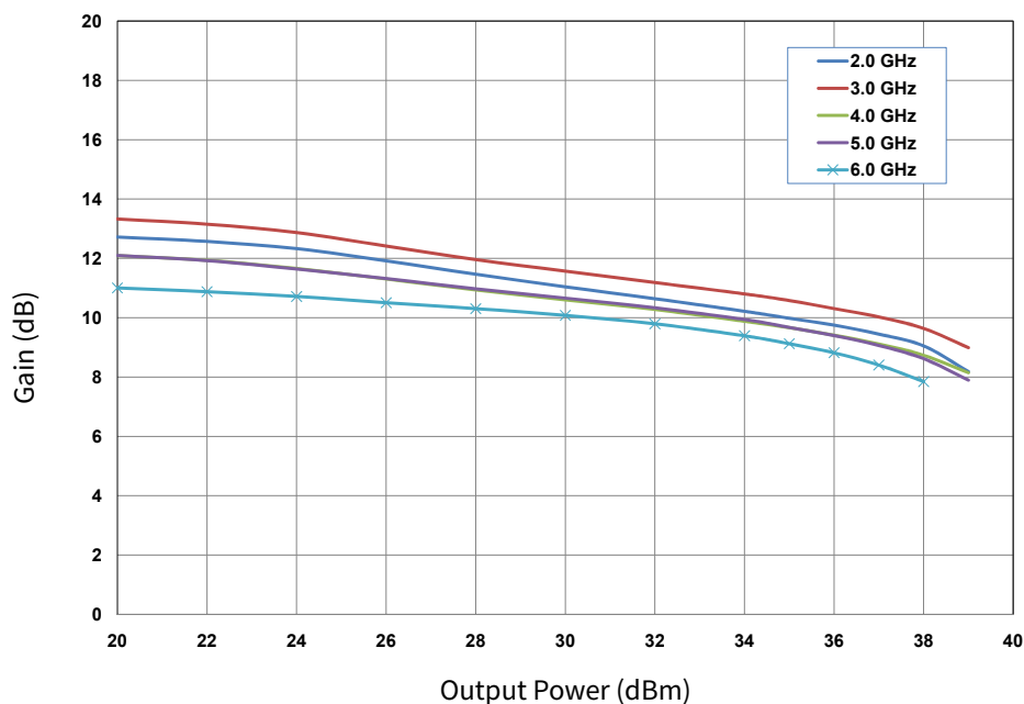
Figure 3. Power Gain vs Output Power as a Function of Frequency of the CGH40006S in the CGH40006S-AMP1 V_{DD} = 28 \text{ V} , I_{DQ} = 100 \text{ mA}
