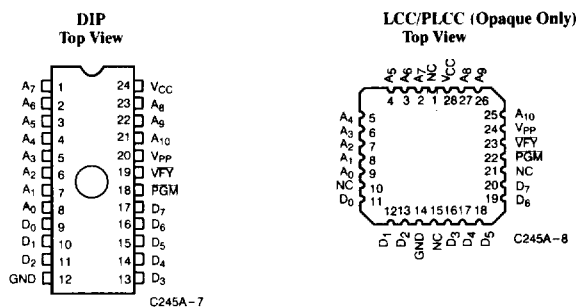
Figure 1. Programming Pinouts
