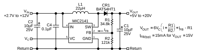
Figure 2. Gain-Boost Configuration
