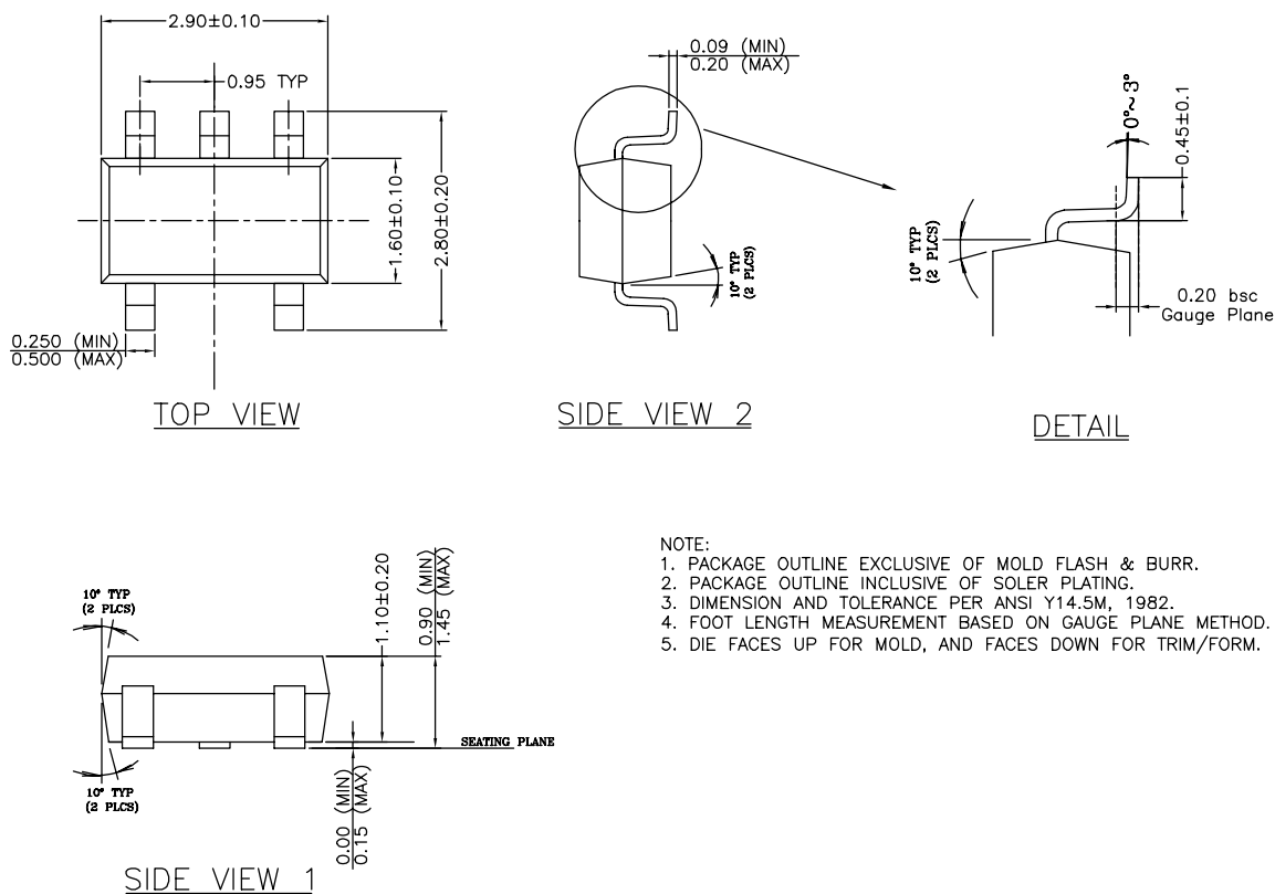
5-Pin SOT23 (M)
