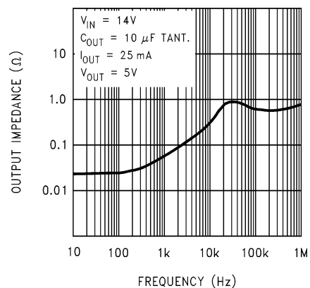
Output Impedance
