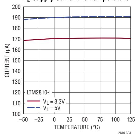
V_L Supply Current vs Temperature
