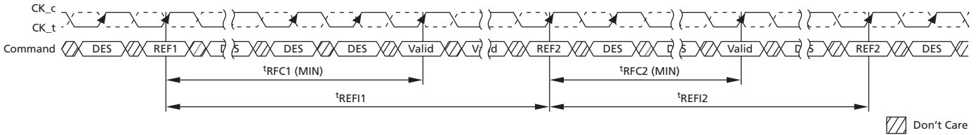
Figure 80: OTF REFRESH Command Timing
