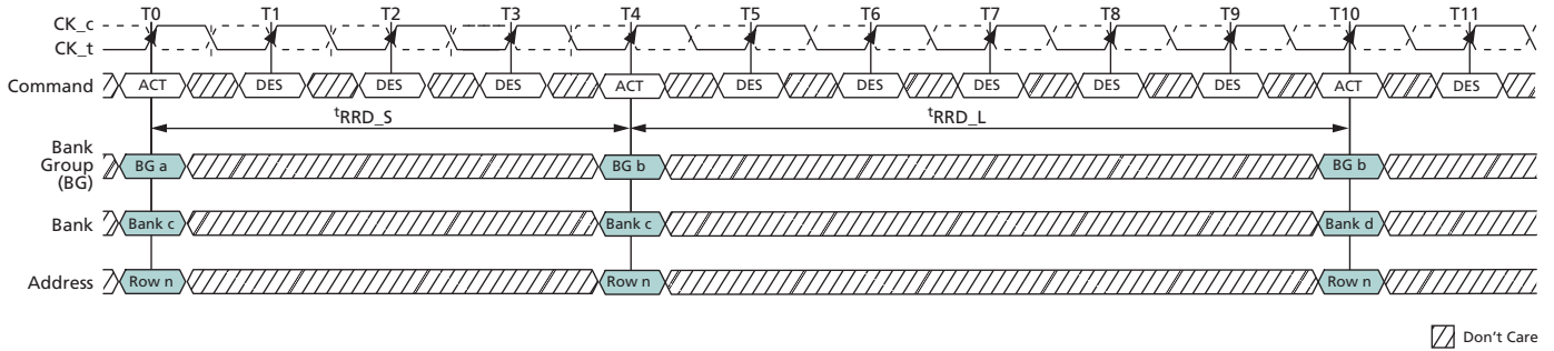
Figure 113: t_{RRD} Timing
