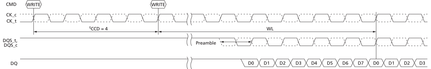
Figure 103: 1 t CK vs. 2 t CK WRITE Preamble Mode, t CCD = 4
