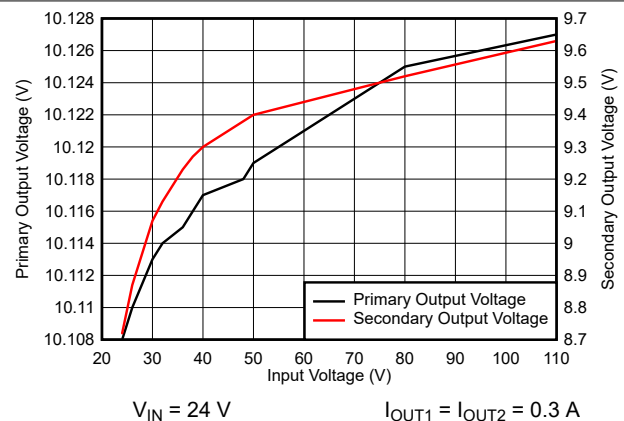
Figure 9-5. Line Regulation
