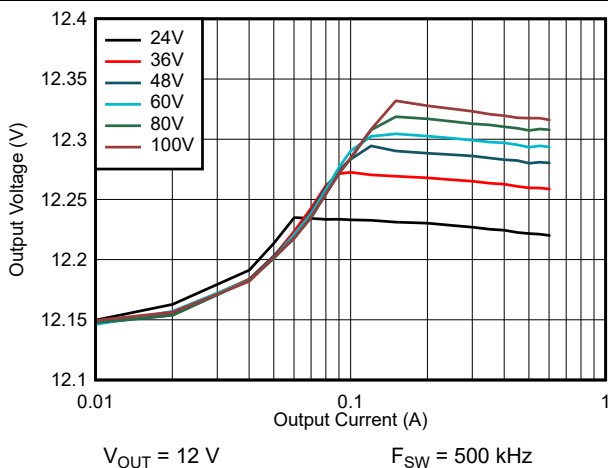
Figure 9-19. Line and Load Regulation: V_{OUT} = 12\text{ V}
