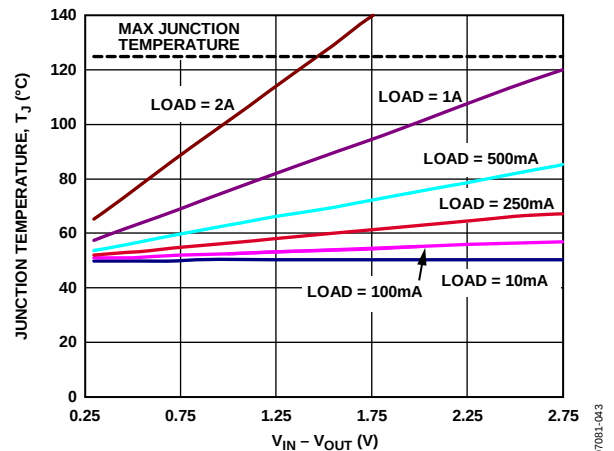
Figure 45. 1000 mm 2 of PCB Copper, T_B = 50^\circ\text{C} , LFCSP
