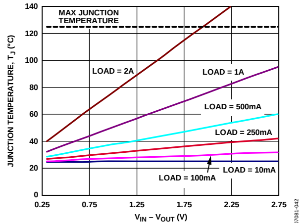
Figure 44. 1000 mm 2 of PCB Copper, T_B = 25^\circ\text{C} , LFCSP
