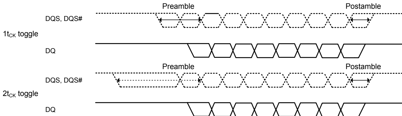
Figure 87. WRITE Postamble
