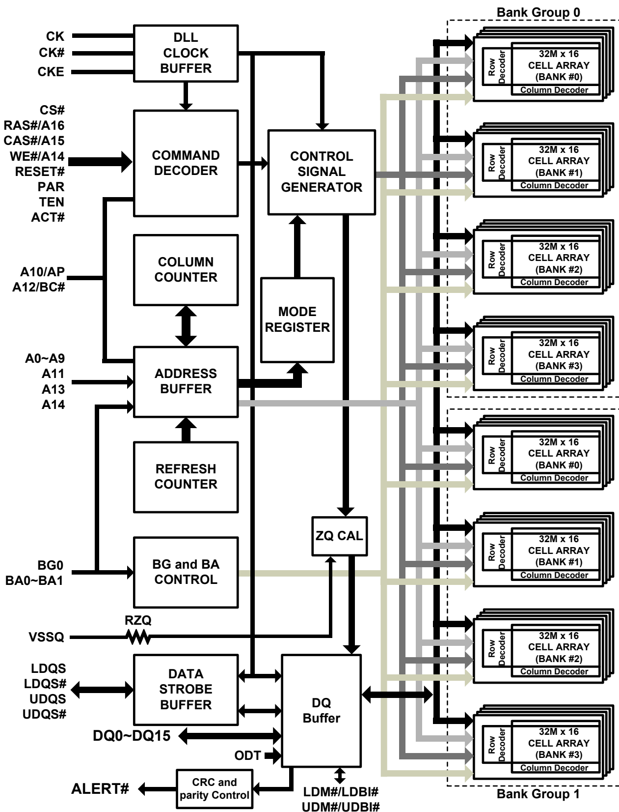
Figure 2. Block Diagram
