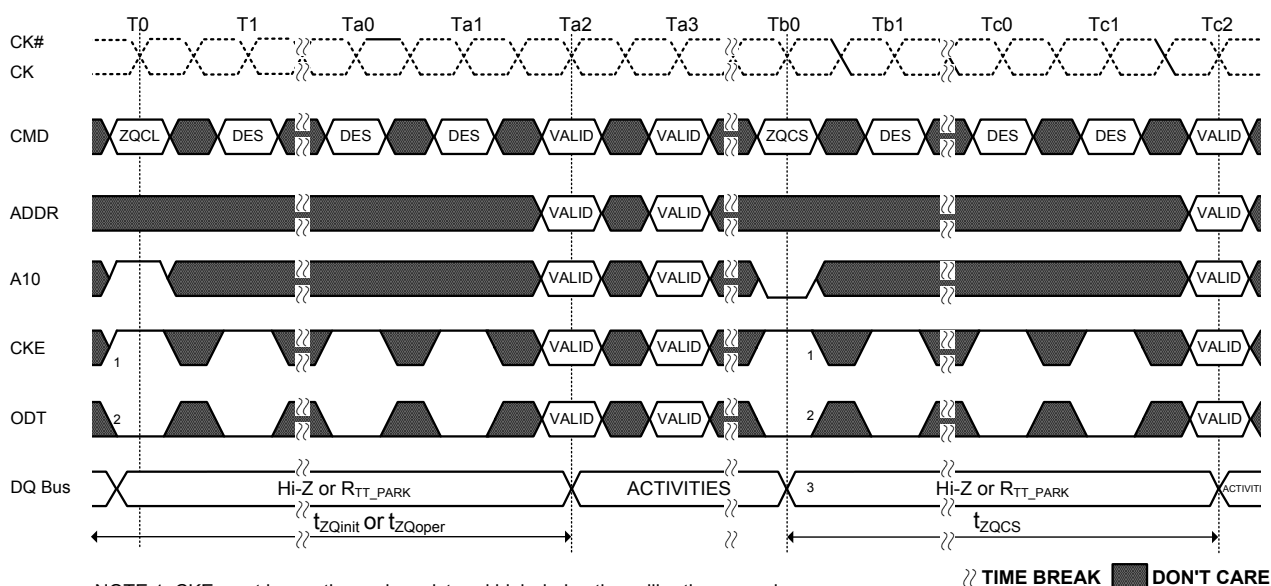
Figure 45. ZQ Calibration Timing
