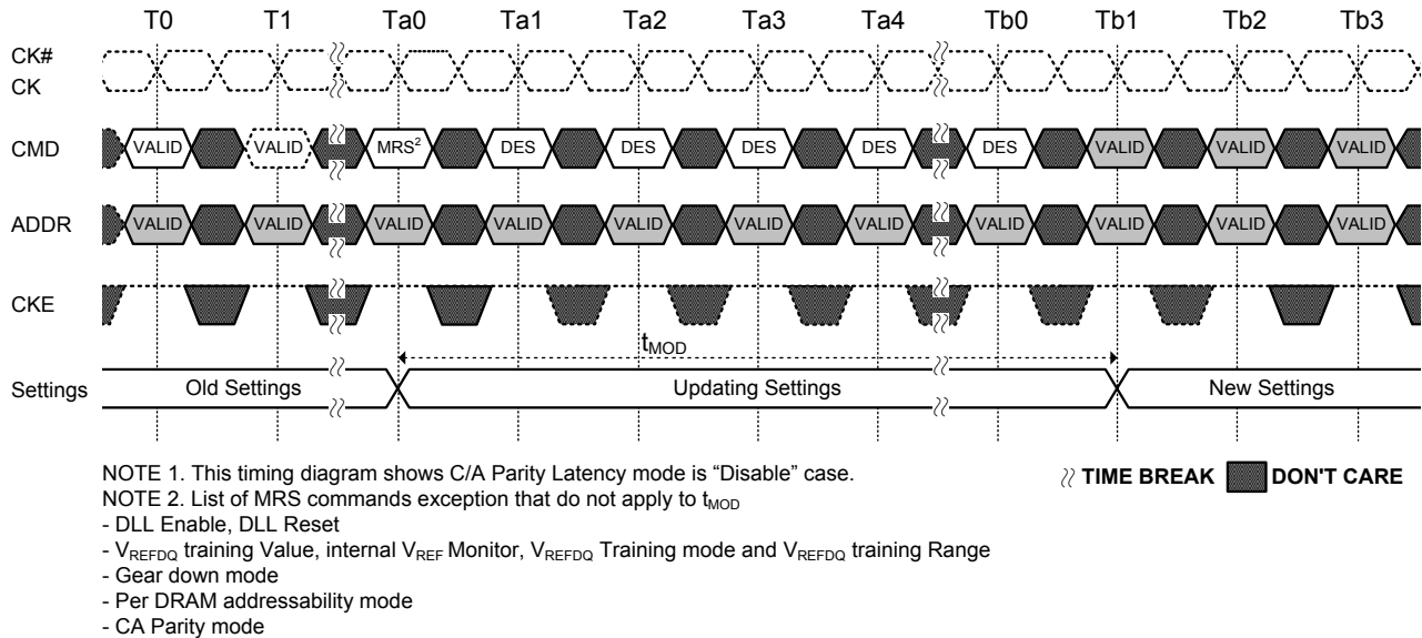
Figure 7. t_{MOD} timing
