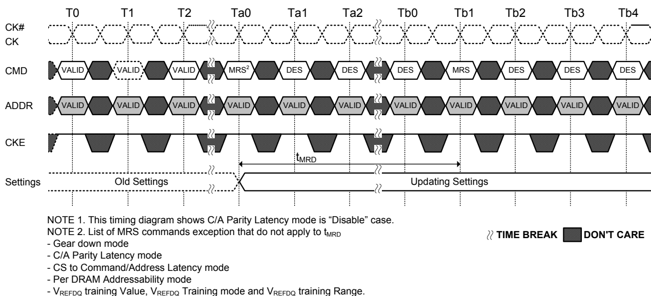
Figure 6. t_{MRD} timing
