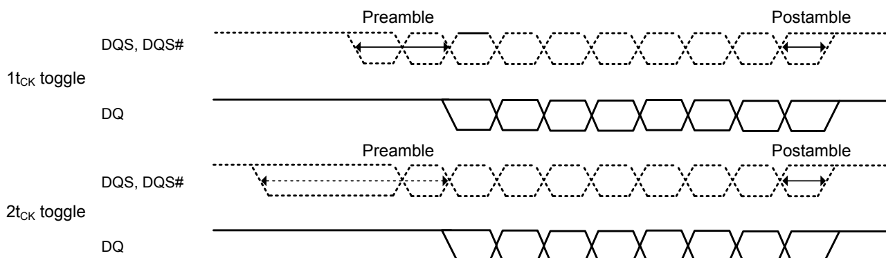
Figure 86. READ Postamble
