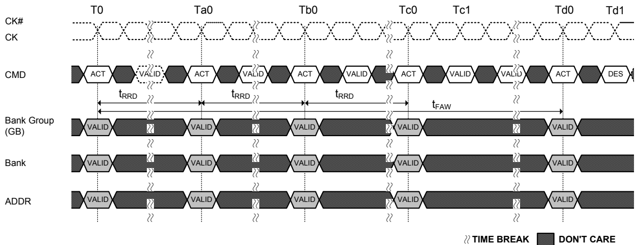
Figure 77. t_FAW Timing
