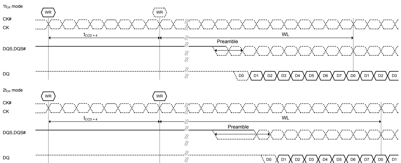
Figure 81. t_{CCD}=4 (AL=PL=0)
