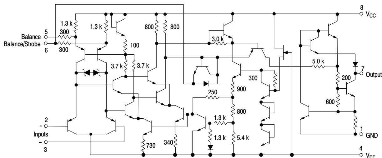
Figure 2. Circuit Schematic
